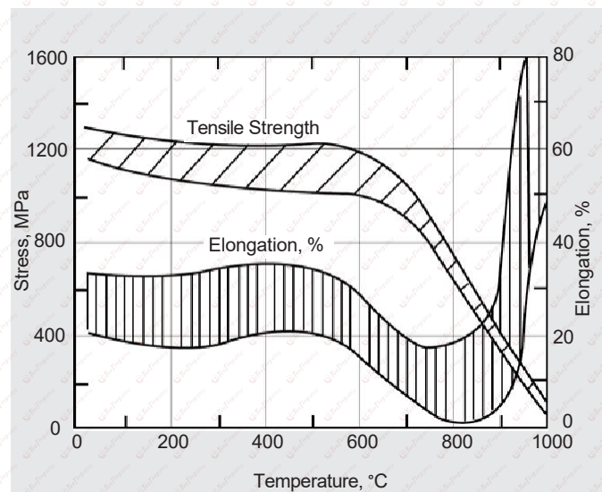
Figure 4. Tensile properties of extruded bar subsequently forged.
